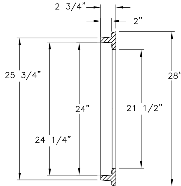
FRAME SECTION
