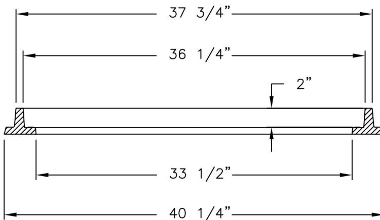
FRAME SECTION
